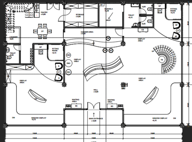
LAYOUT LT.1
